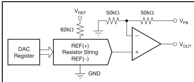
Figure 45. DAC8550 Architecture
