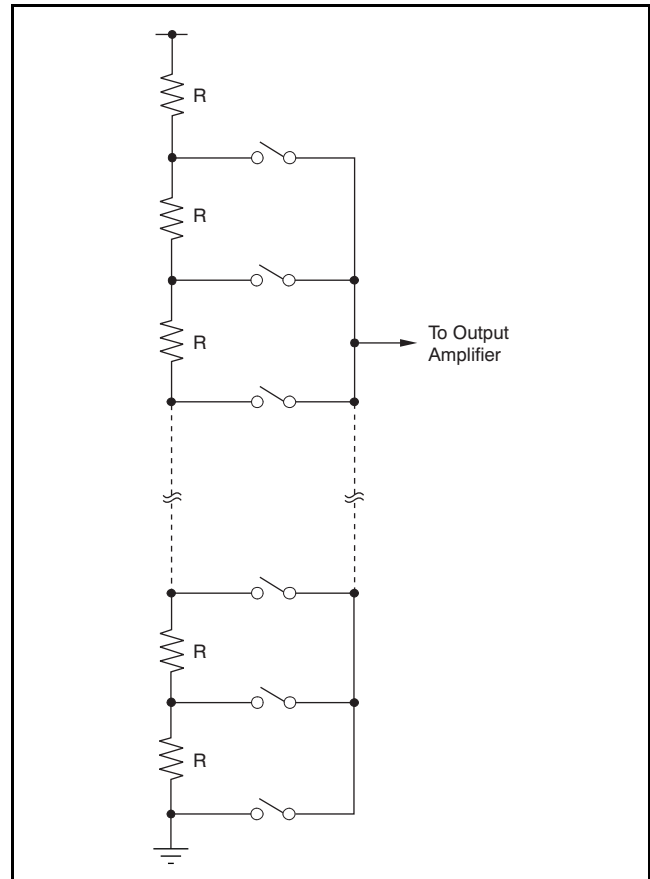
Figure 46. Resistor String
