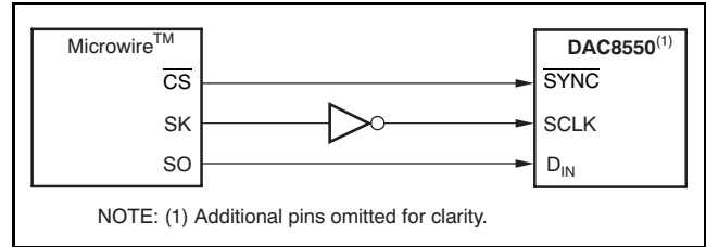
Figure 51. DAC8550 to Microwire Interface
